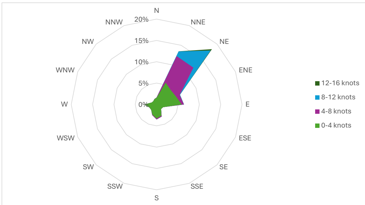
Figure 4-19: Windrose Diagram for Hampden, St. James (January 2022 - 2024)
