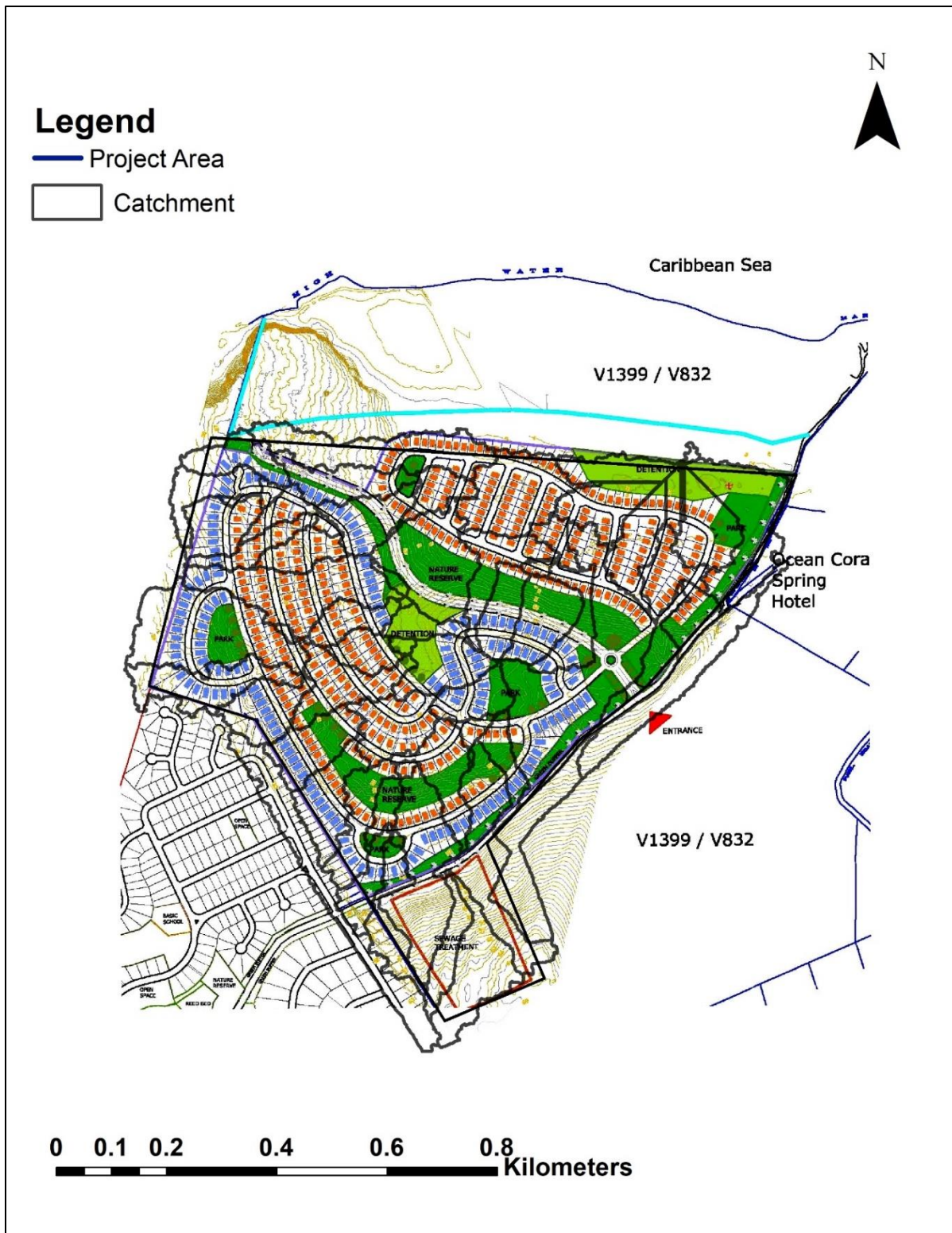
Figure 4-11: Map showing the different catchments and the draft layout plan for the development.
